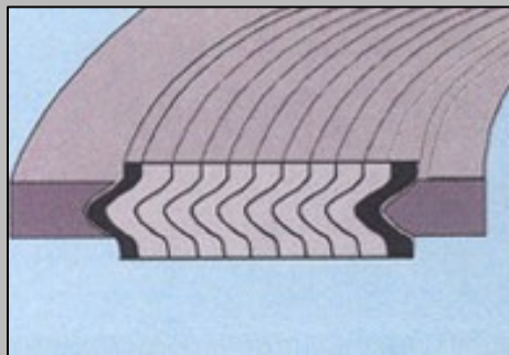
STYLE LG-13-IR: SPIRAL WOUND with INNER and OUTER RING
